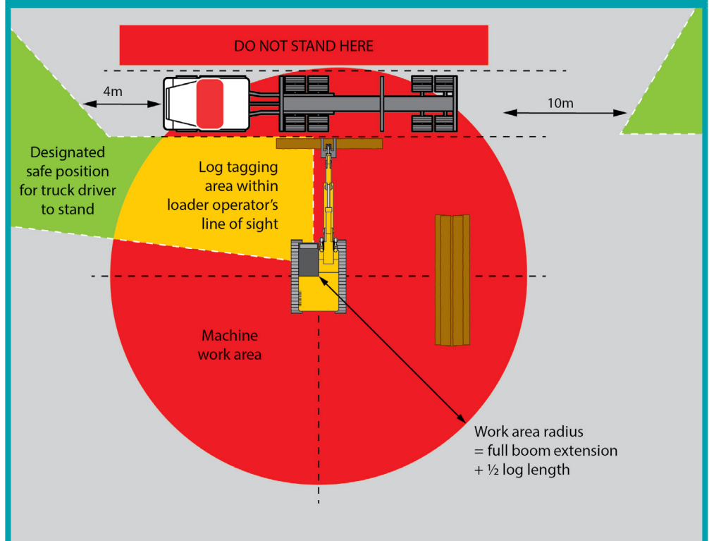
FIGURE 1 An example of a safe work area in a log landing
